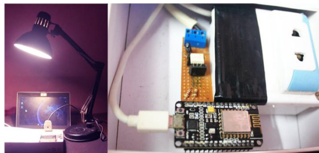
Figure 4. Prototype of the IoT Switching Model
